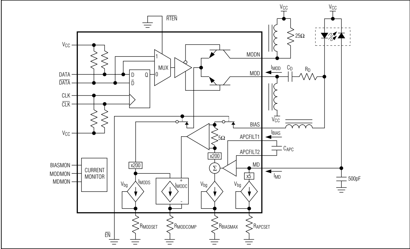
Figure 3. Functional Diagram
