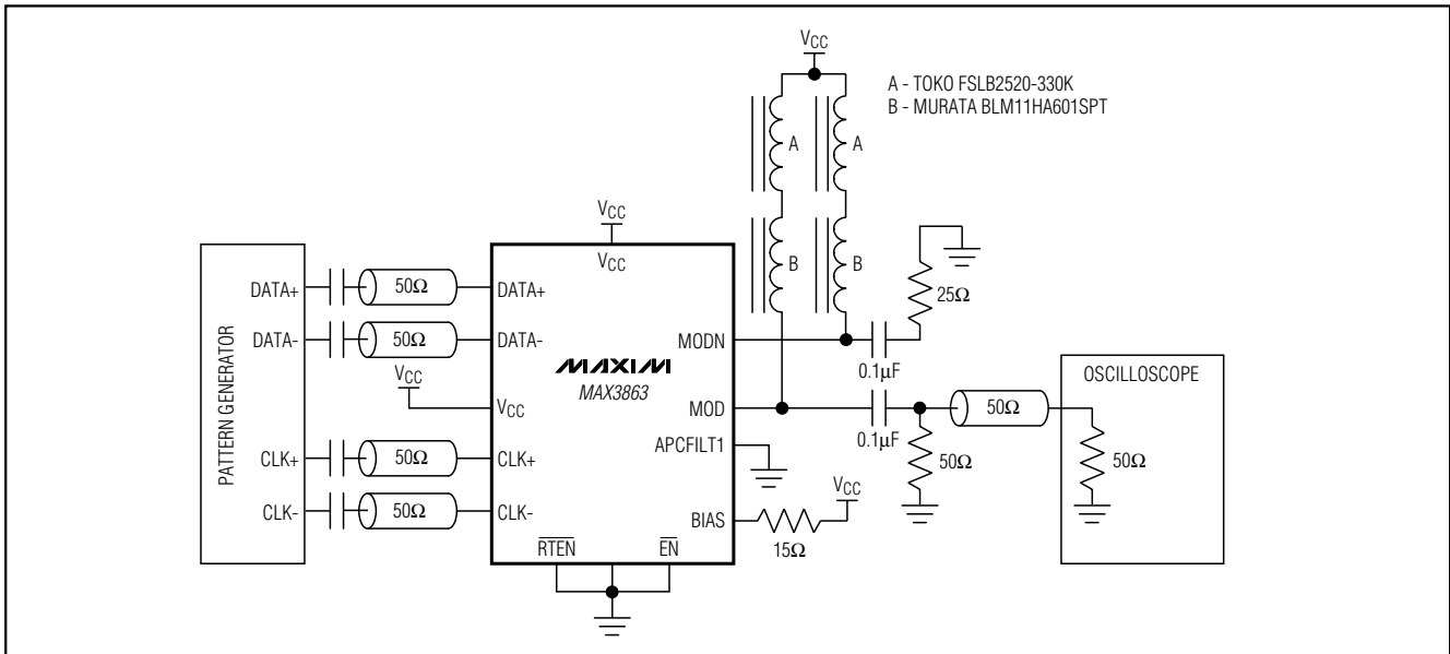
Figure 1. AC Characterization
